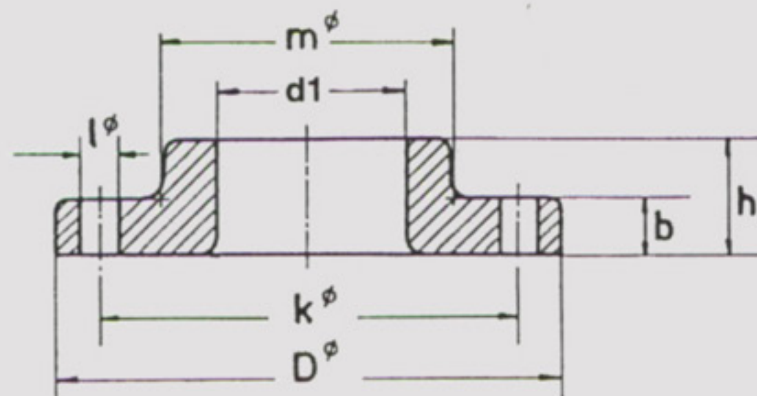
Stainless Steel lap-joint flanges FF 300 lbs according to ASTM A182/ANSI B16.5
